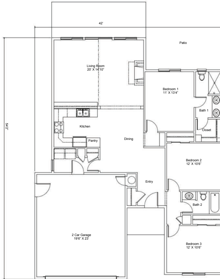
Silverbrook Estates-Plan 6 Floor Plan Study Scheme 5 1394 sq.Ft. Livable
